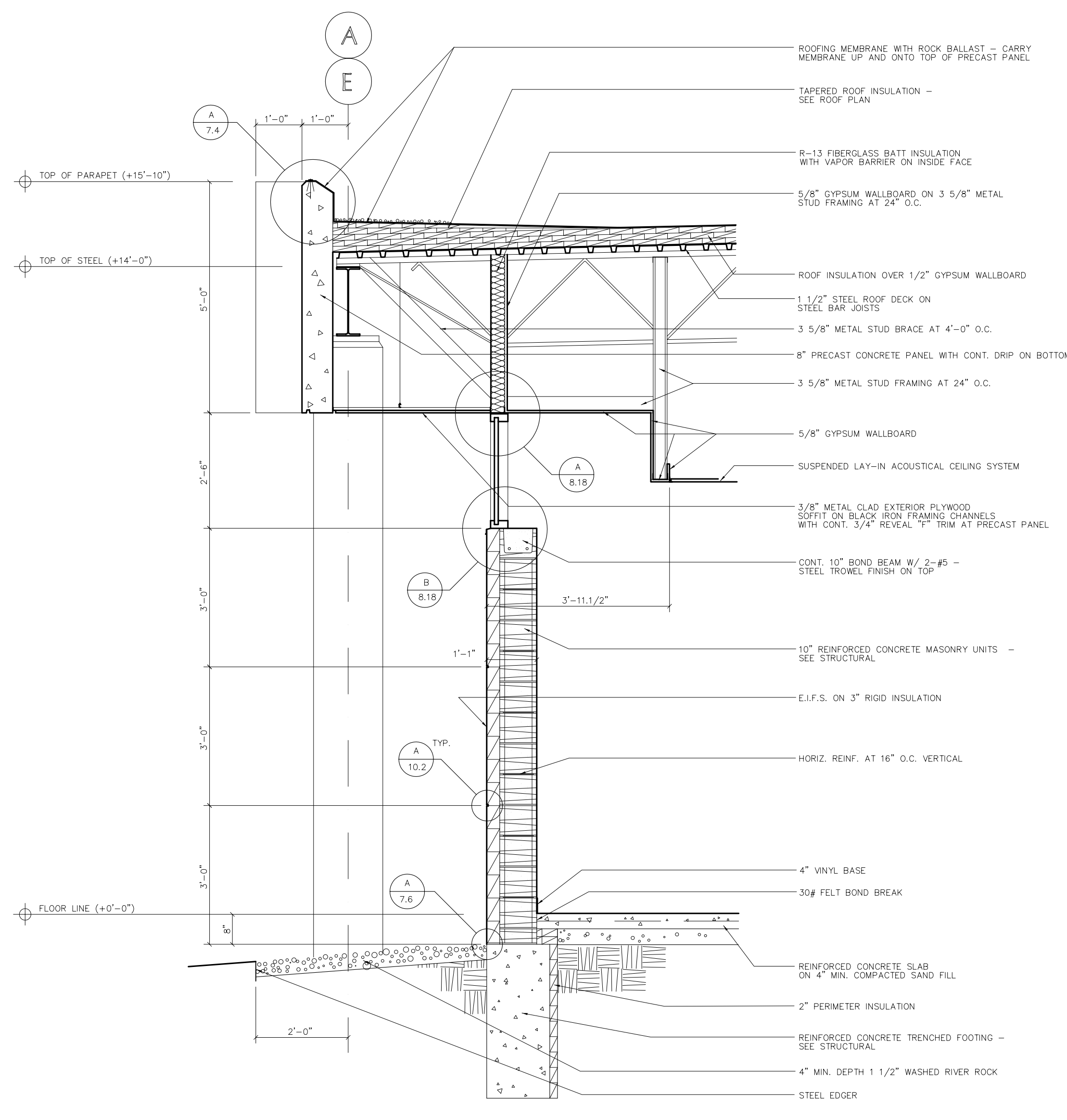
B WALL SECTION 1/2"x1'-0"
