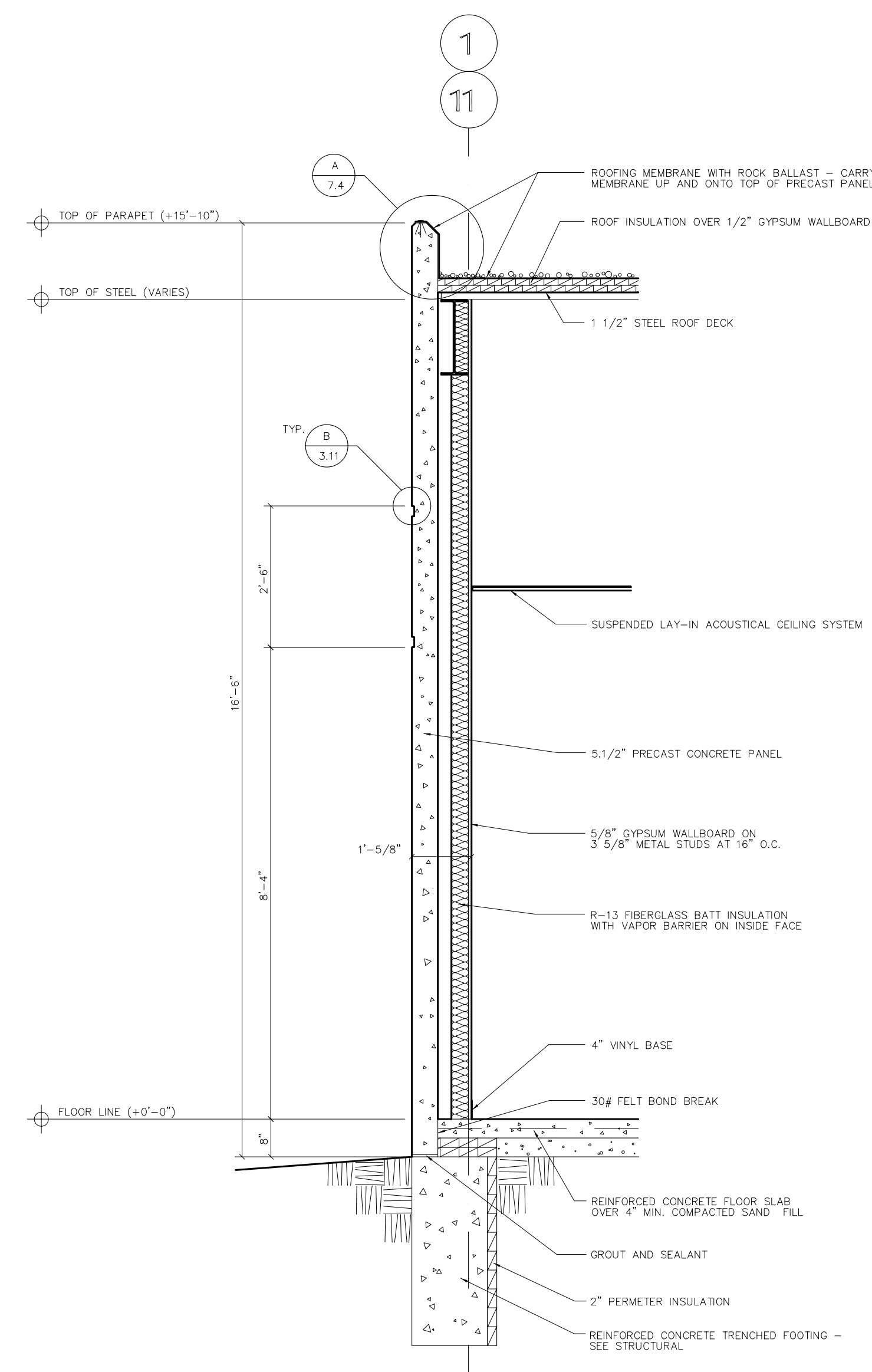
C WALL SECTION 1/2"x1'-0"
