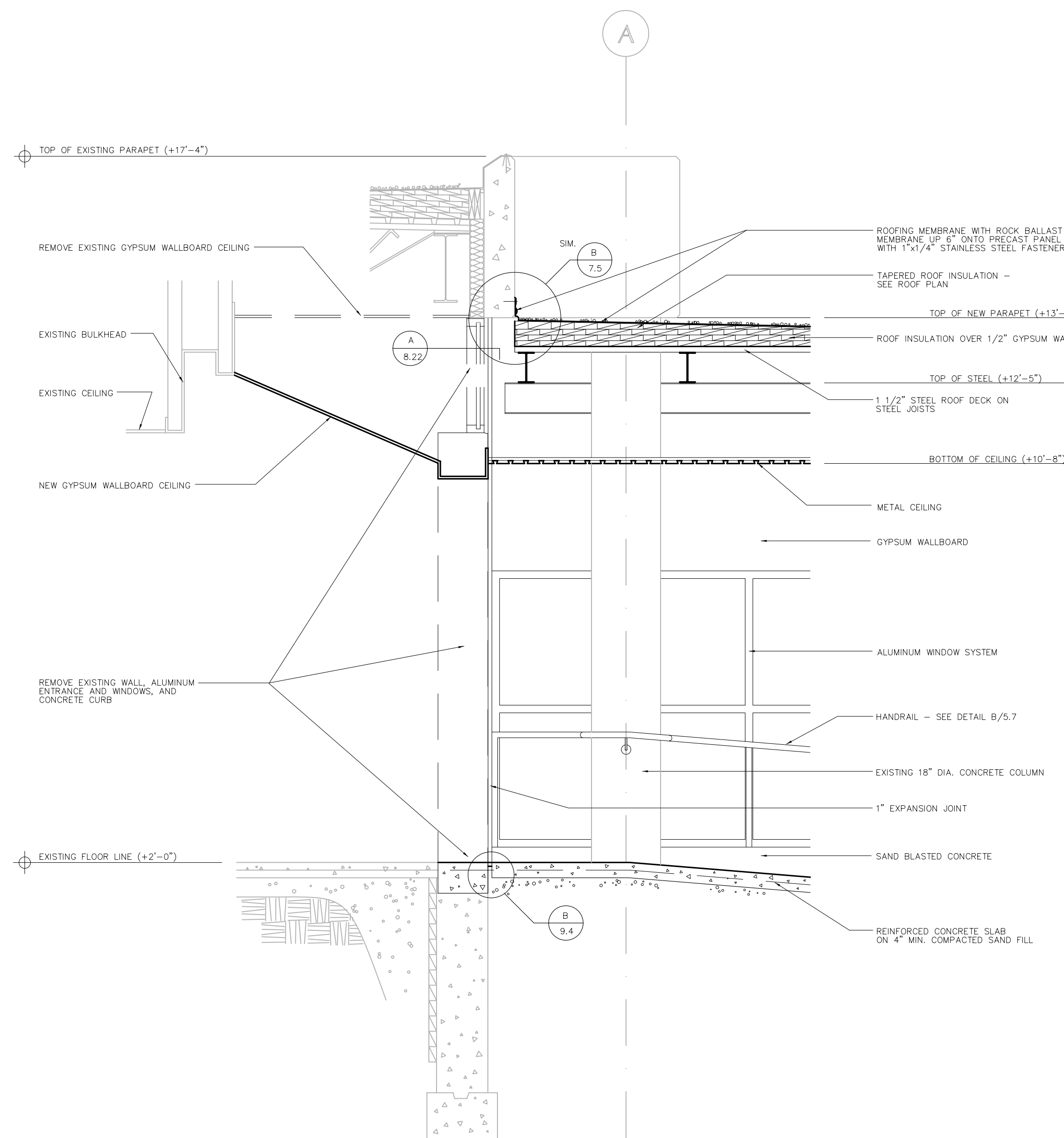
B WALL SECTION 1/2"x1'-0"
