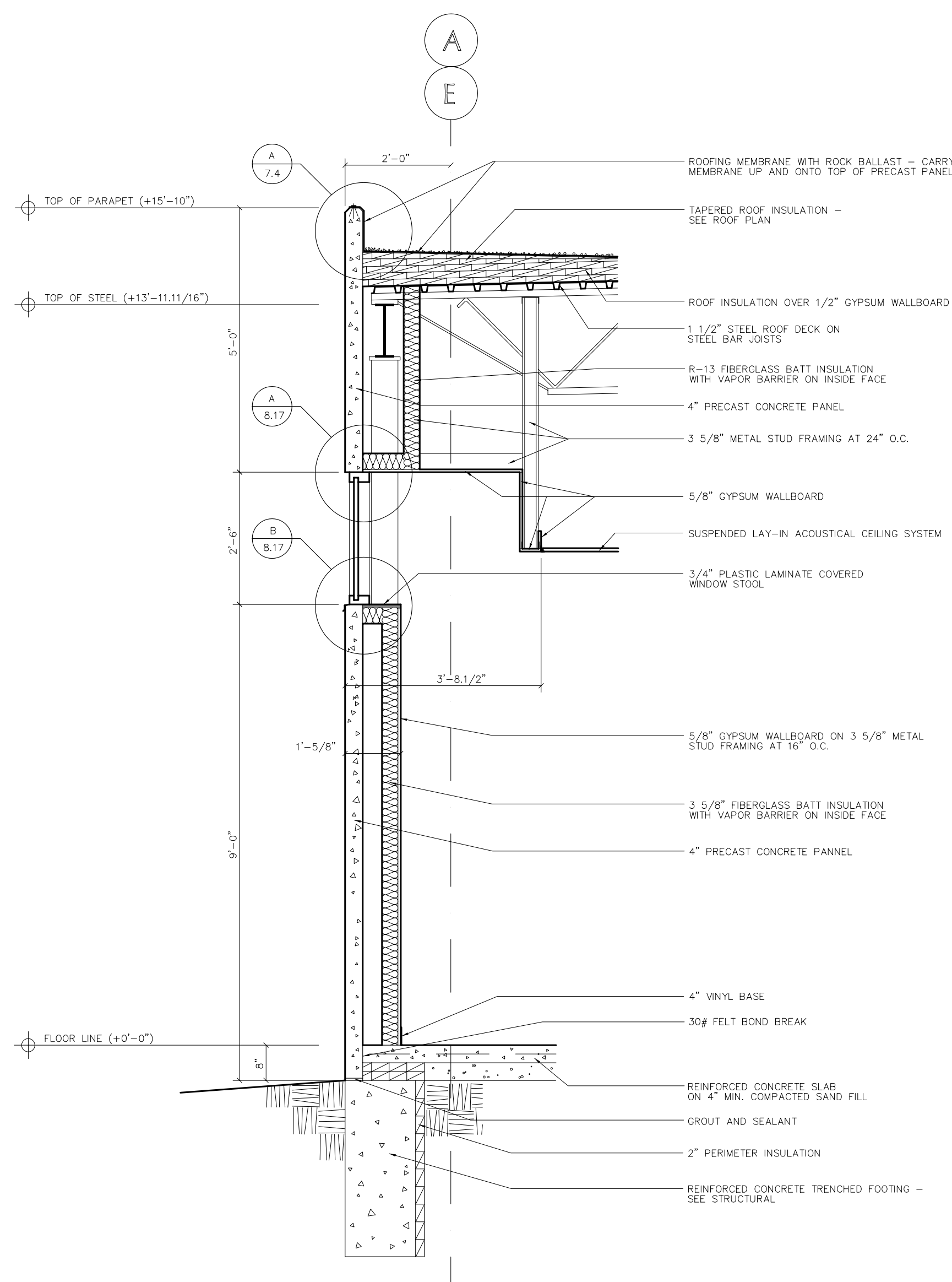
A WALL SECTION 1/2"x1'-0"
