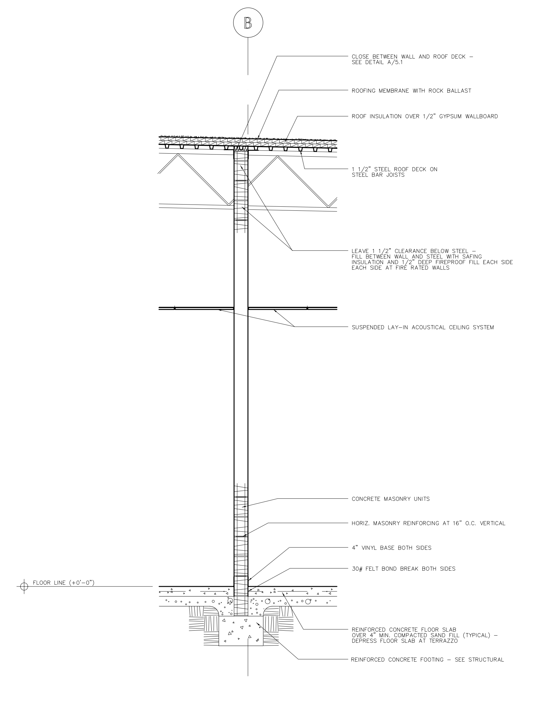
D WALL SECTION 1/2"x1'-0"
