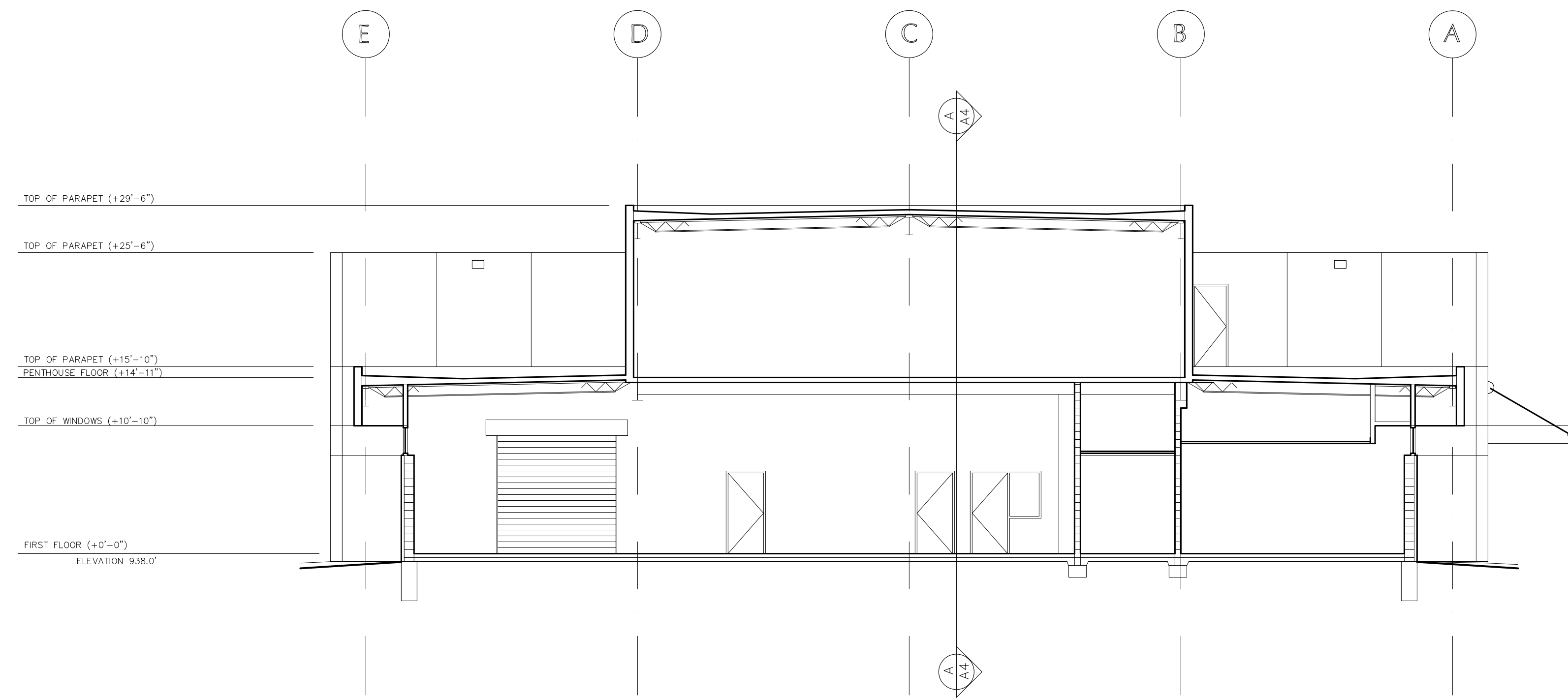
A BUILDING SECTION 1/8" = 1'-0"
