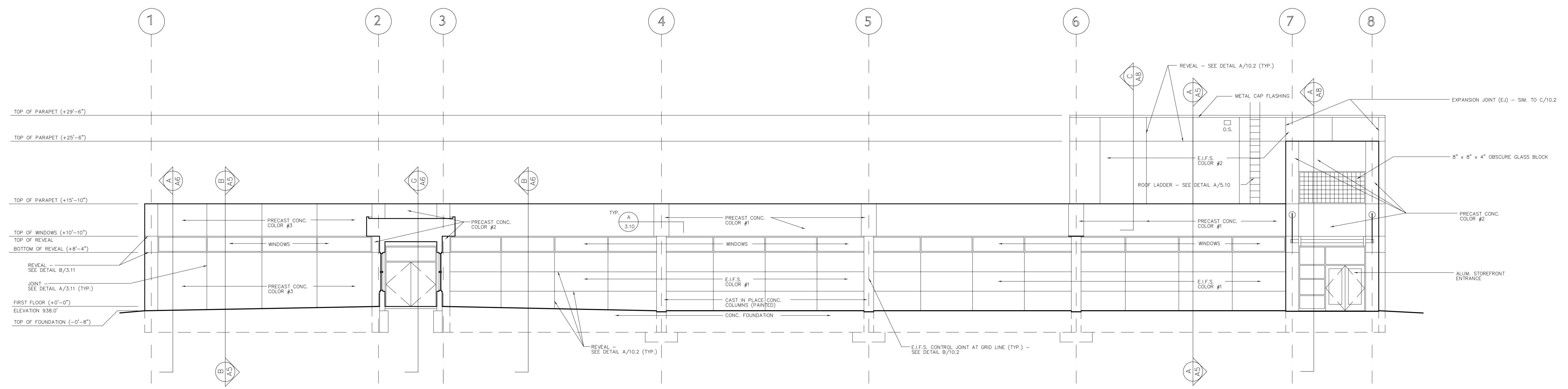
WEST ELEVATION 1/8" = 1'-0"
