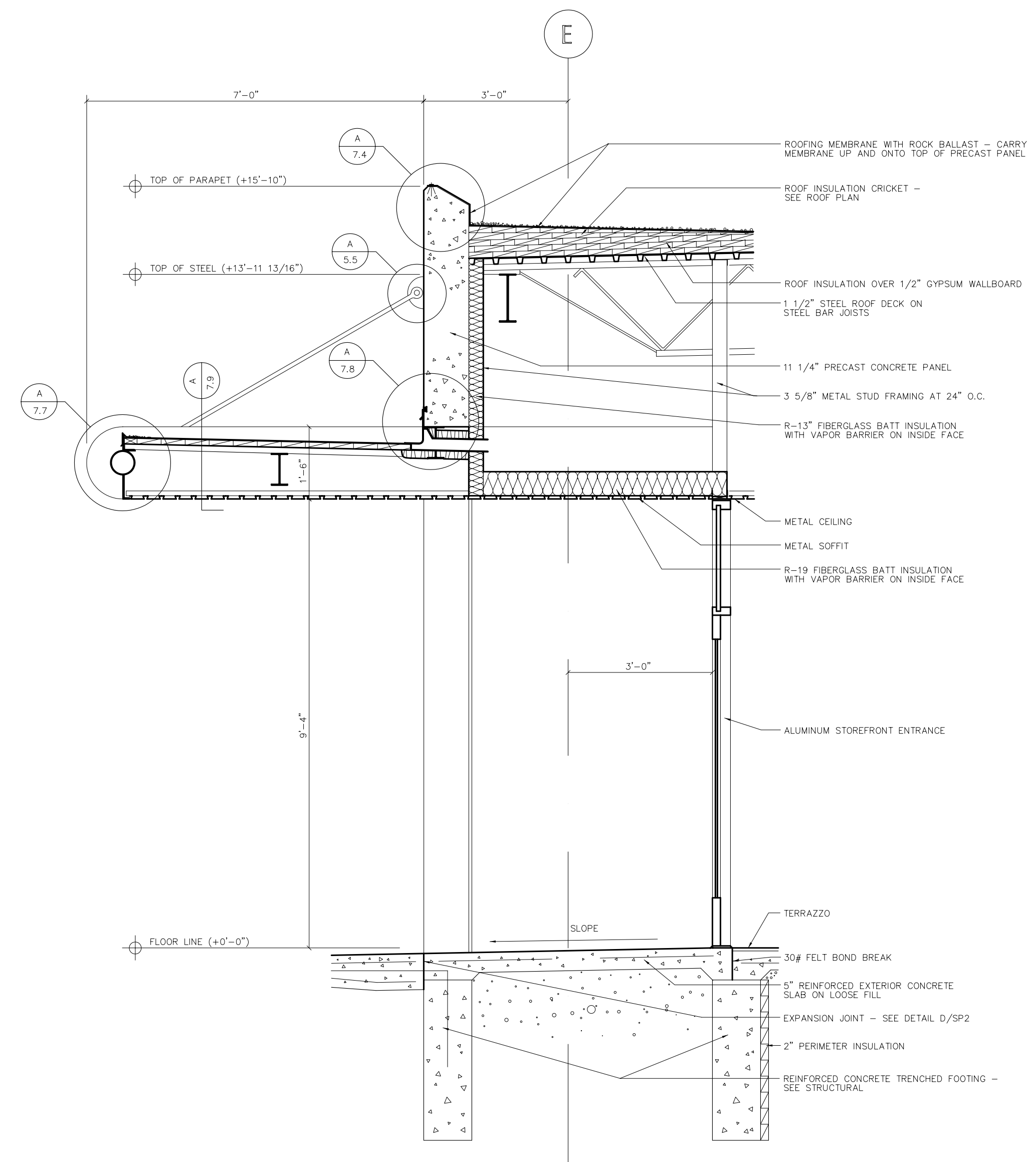
D WALL SECTION 1/2"-1'-0"
