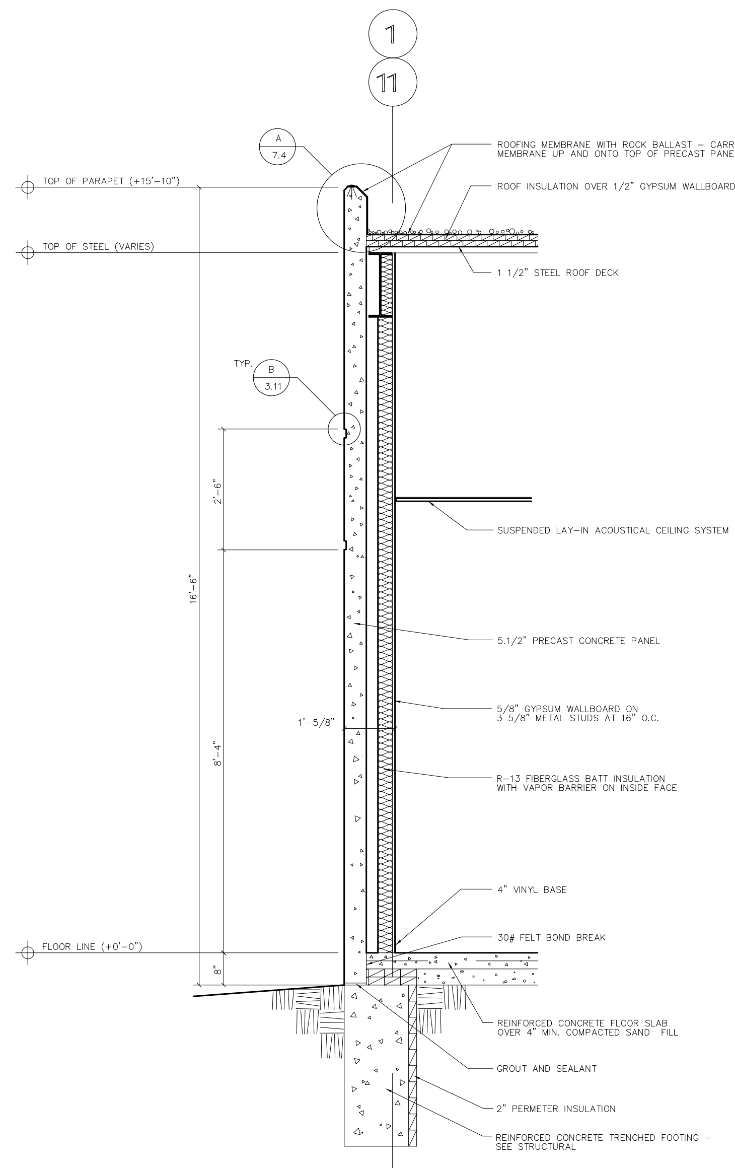
C WALL SECTION 1/2"-1'-0"
