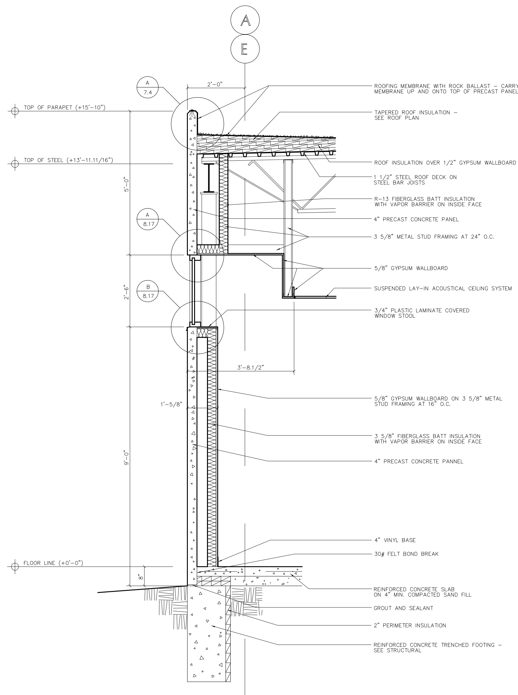
A WALL SECTION 1/2"-1'-0"
