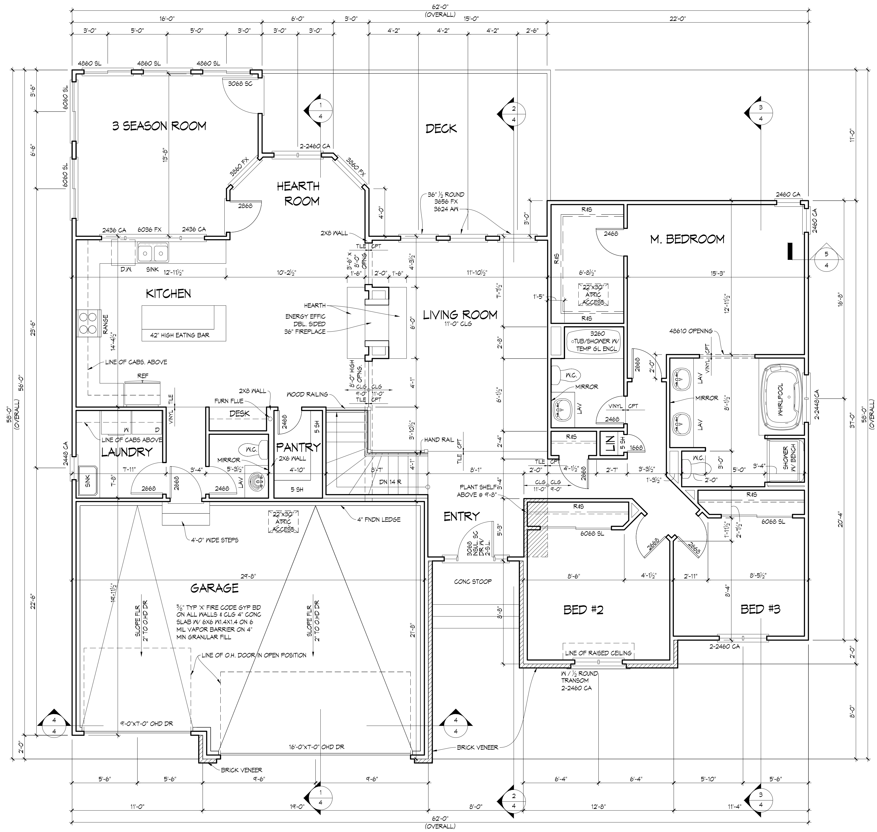
1 MAIN FLOOR PLAN SCALE: 1/4" = 1'-0"
