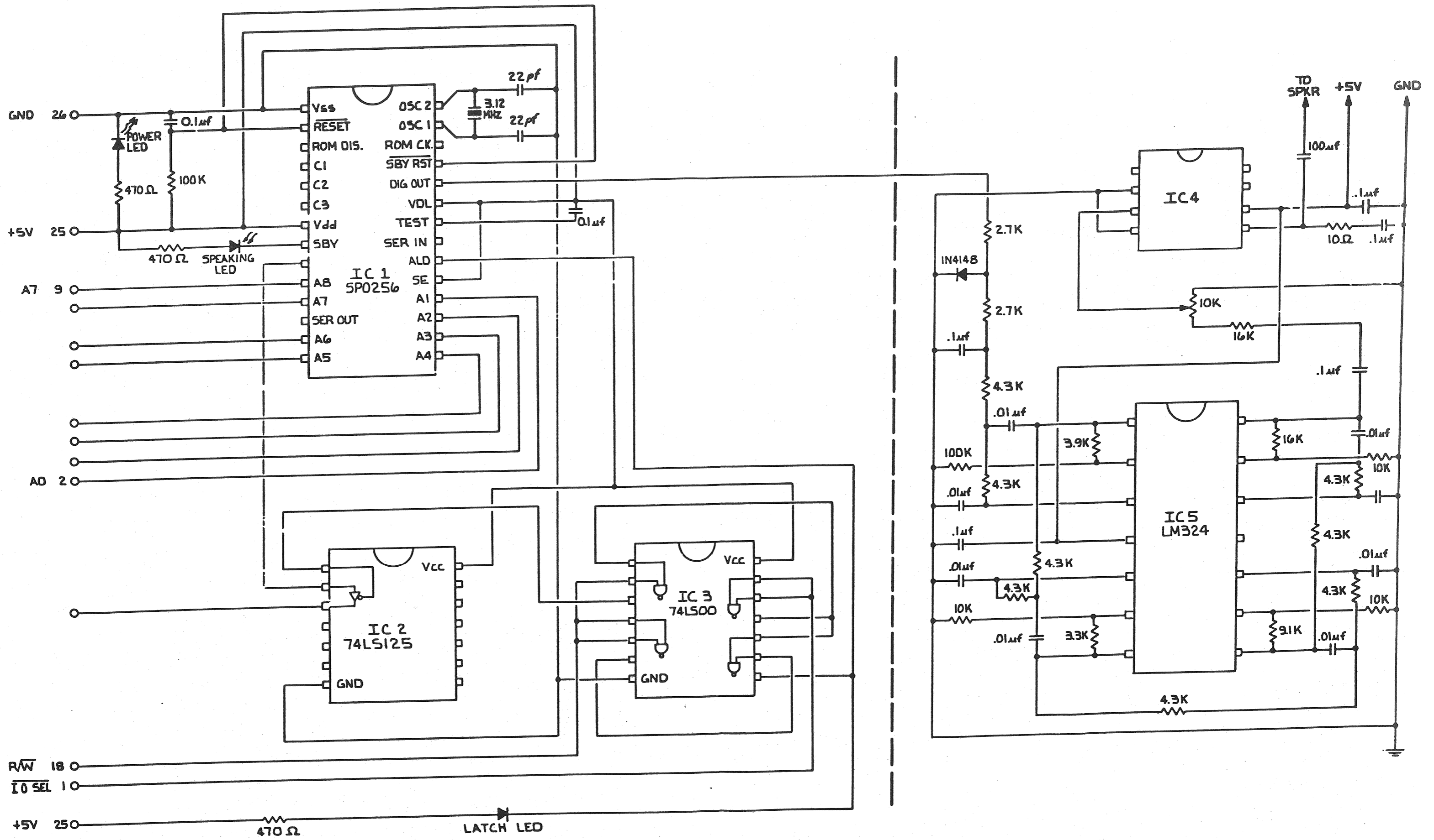
FIGURE 8.03.C - SCHEMATIC OF COMPLETE SYNTHESISER
